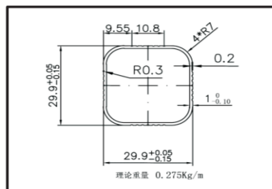
DY-Rungs 29.9x29.9 SQB014
