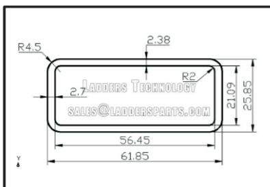
FML 62x26x2.3MM
