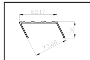
DY-STEP PROFILE
