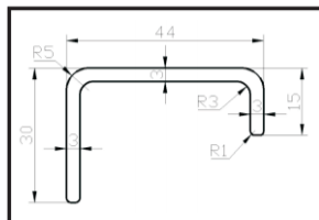
DY-REAR RAIL PROFILE
