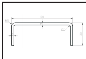
DY-FRONT RAIL PROFILE
