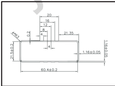
DY-Side Profile SQB017
