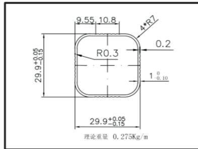
DY-Rungs 29.9x29.9 SQB014
