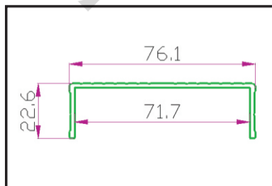
前立柱 Front Rail Profile
