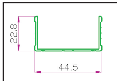
后立柱 Rear Rail Profile
